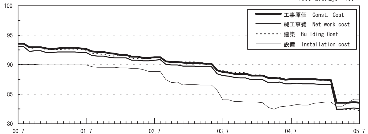
図-4 No. 32 個人住宅 W 125㎡ fig. 4 Individual house
