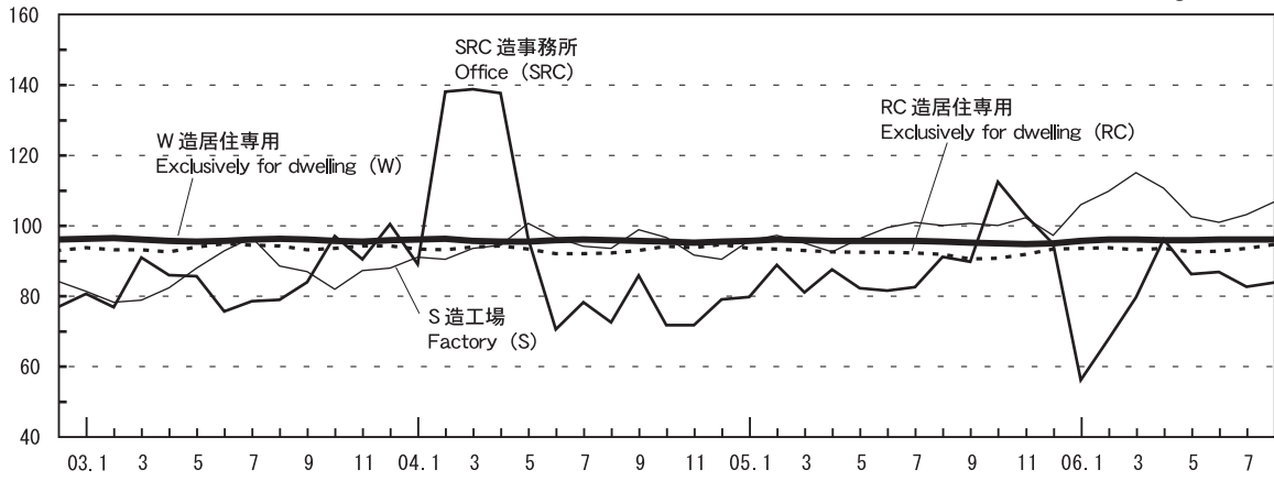
図-7 主な構造・用途の予定工事費単価指数 fig.7 Estimated construction price per sq.m. by Statistics on Building Construction Started 平成7年平均=100 1995 average=100
