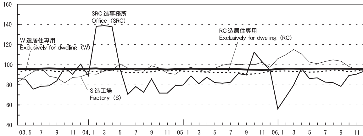
図一七 主な構造・用途の予定工事費単価指数 fig.7 Estimated construction price per sq.m. by Statistics on Building Construction Started
