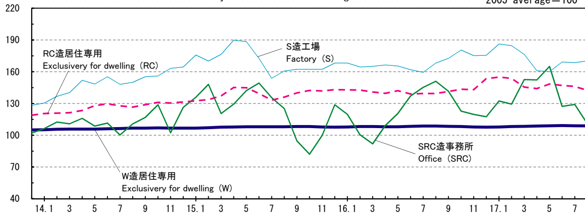
図－７ 主な構造・用途の予定工事費単価指数 fig.7 Estimated construction price per sq.m. by Statistics on Building Starts
